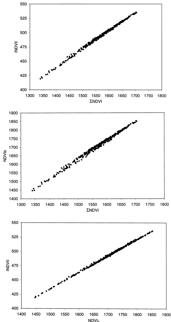
Fig. 1. Scattergrams of the pairwise linear relationships between the three analysed cumulative vegetation indices: (a) \Sigma\text{NDVI} vs. |\text{NDVI}| , (b) \Sigma\text{NDVI} vs. \text{NDVI}_S , (c) \text{NDVI}_S vs. |\text{NDVI}| .
