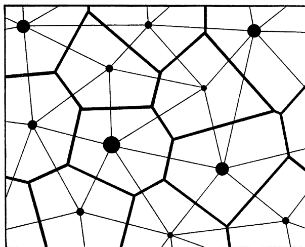
Fig. 2. The Delaunay triangulation (fine lines) and Dirichlet tessellation tiles (solid lines) for a subset of points from a larger population.
