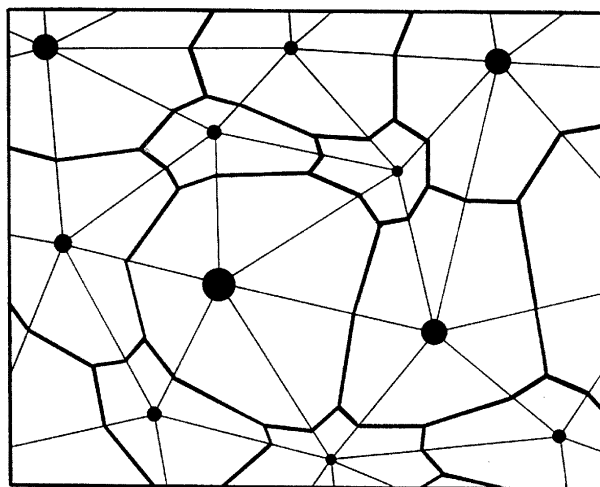
Fig. 7. Delaunay triangulation (fine lines) and the weighted Fraser tessellation (solid lines) for the point pattern shown in Fig. 2. Weights are proportional to circle diameter.
